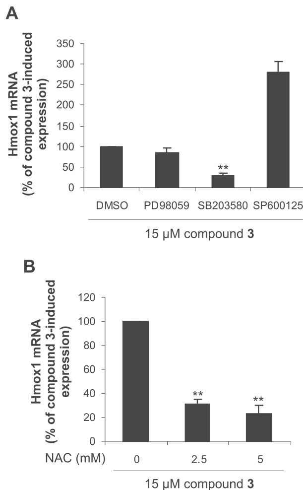
Fig. 5. Effect of MAPK inhibitors and N -acetyl-L-cysteine (NAC) on 7- O -galloylquercetin (compound 3 )-induced Hmox1 gene expression in RAW264.7 cells. (A) Cells were pretreated for 30 min with 0.1% DMSO (control), 15 μM PD98059, 15 μM SB203580 or 30 μM SP600125 and then incubated in the absence or presence of 15 μM 3 for an additional 6 h. (B) Cells were pretreated for 30 min with 2.5 or 5 mM NAC and then incubated in the absence or presence of 15 μM 3 for an additional 6 h. The levels of Hmox1 mRNA were determined by quantitative real-time PCR and normalized to Gapdh mRNA. Results are expressed as the percentage of compound 3 -induced Hmox1 mRNA expression. Data are means ± SD of three experiments. ** p < 0.01, significantly decreased versus 3 in the absence of MAPK inhibitors or NAC.
